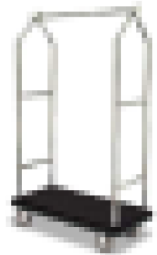
2543 Specialty Luggage Cart with polished stainless steel frame 111 cm x 56 cm x 182 cm 57kg
